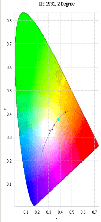
▼ CHROMATICITY DIAGRAM:
